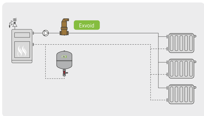
Exvoid Brass system – diagram
