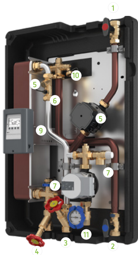
Reflex Hydroflow L – XL freshwater station models
