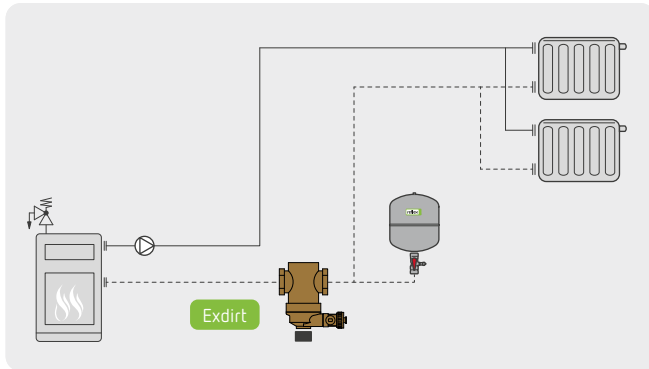
Exdirt Brass system – diagram
