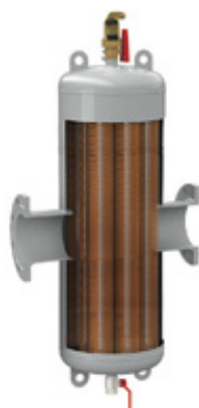
Extwin HC flange connection cutaway model
