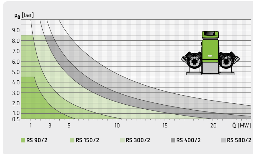
Reflexomat with two compressors
