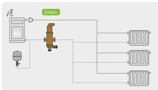
Extwin brass system – diagram
