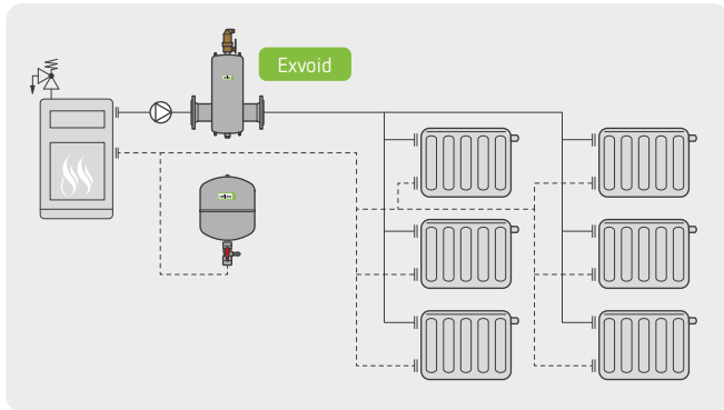
Exvoid steel system – diagram
